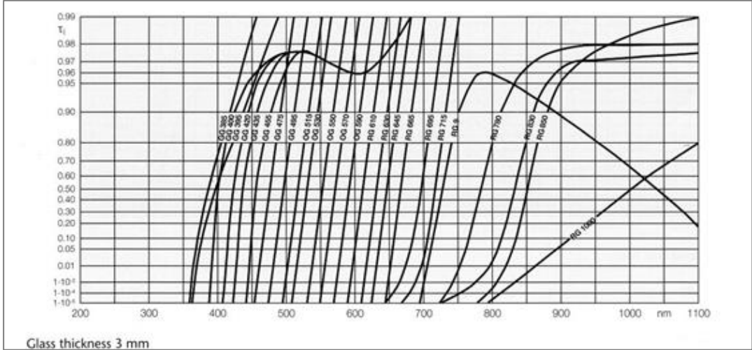
Figure 8-1: Optical Transmission Spectra of Cadmium-based Glass Filters
