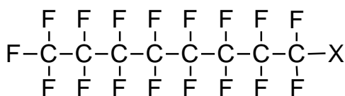
Figure A.1- 2: Chemical structure of PFOA (top) and PFOA-related substances
