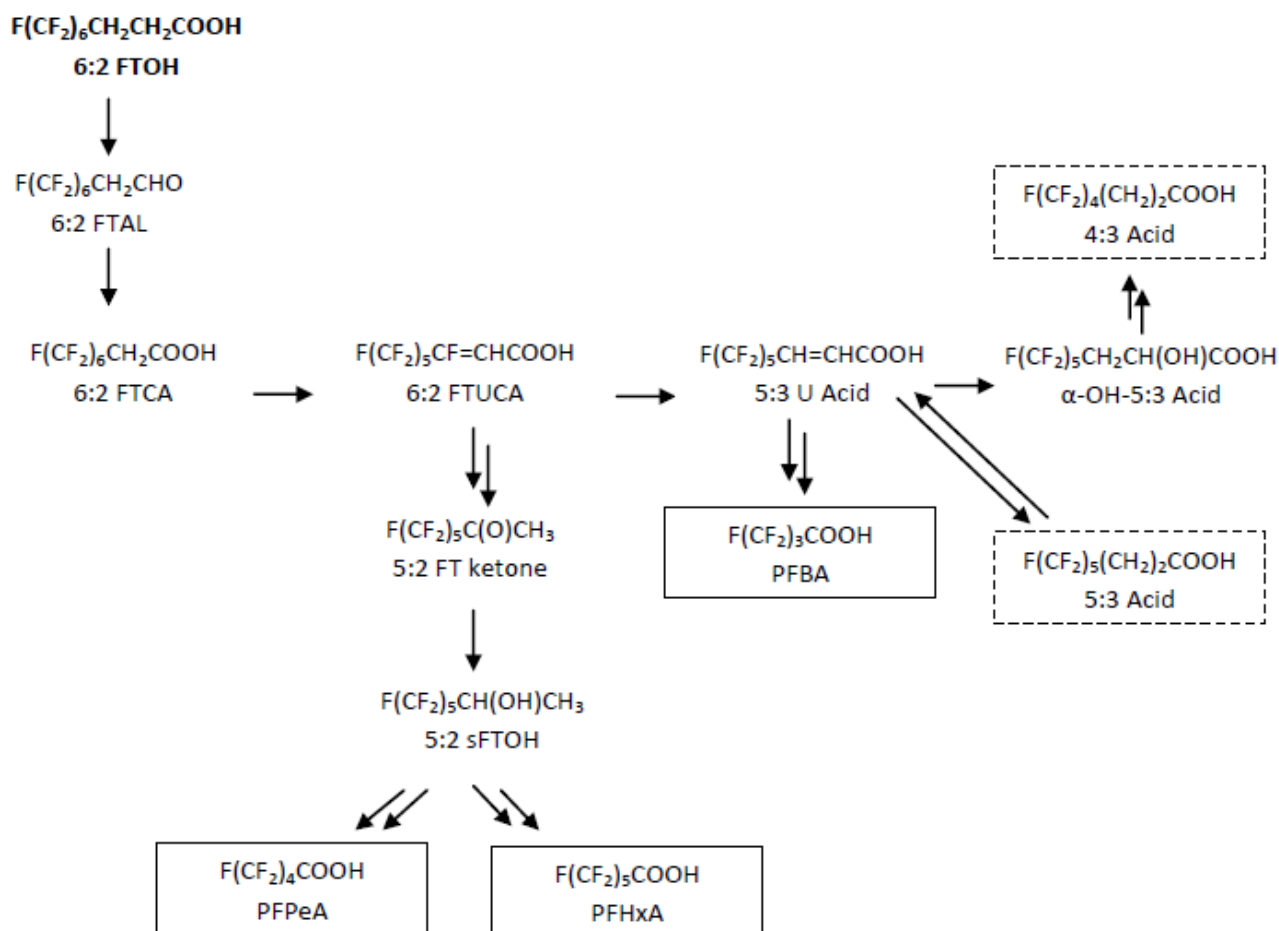
Figure C.2-1: Proposed 6:2 FTOH aerobic biodegradation pathways. The single arrows indicate transformation steps based on observed transformation product and the double arrows indicate multiple transformation steps (based on (Zhao et al., 2013a)).
